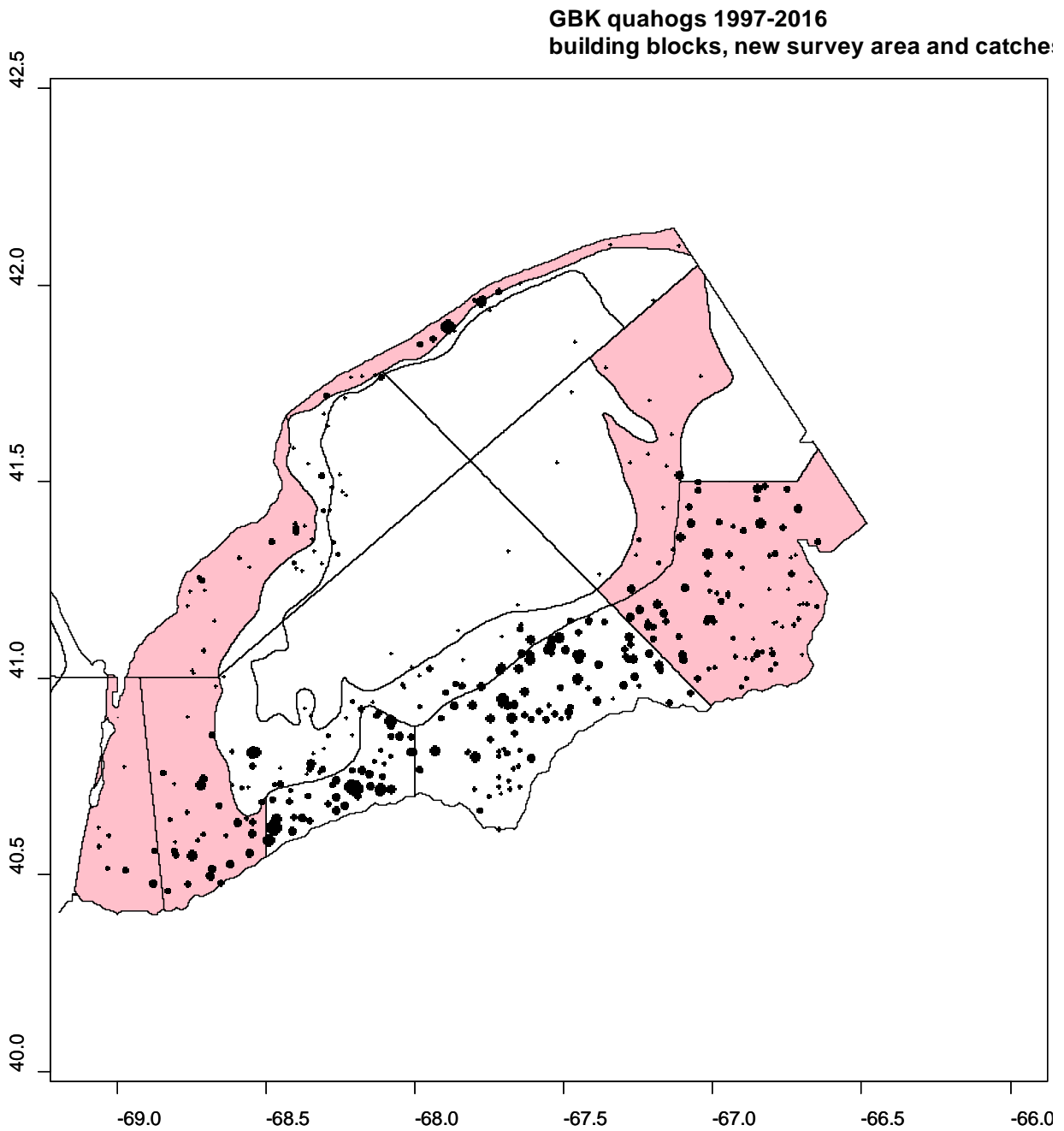
Figure 10. New building blocks (dark lines) and survey area based on the 1% rule for ocean quahogs ( Arctica islandica ) on Georges Bank (GBK), with survey data from 1997-2016 (rescaled to same annual mean). Hollow symbols show stations with zero catch. Solid symbols show location amount and location of catches.
