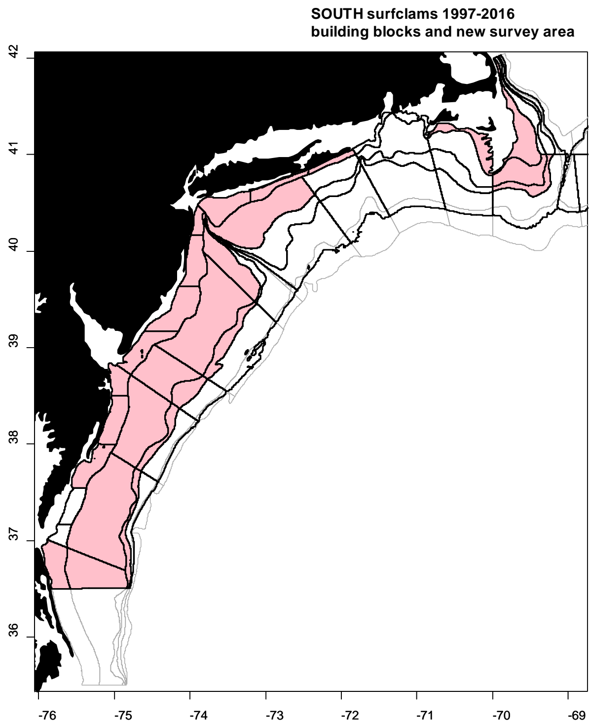
Figure 11. New building blocks (dark lines) and survey area based on the 1% rule for surfclams ( Spisula solidissima ) in the southern areas. Current survey strata boundaries are shown with the thin line.
