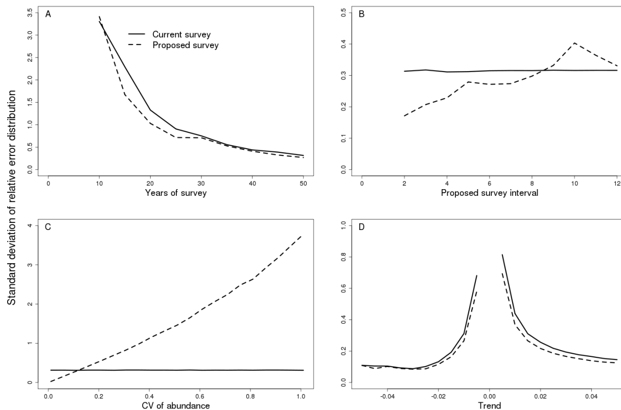
Figure 24. Sensitivity testing for potentially important population parameters for Georges Bank (GBK) ocean quahogs ( Arctica islandica ). The y-axis in each case shows the standard deviation of the distribution of the relative errors shown in Figure 3.16. The dashed line represents the proposed survey, and the solid line represents the current survey.
