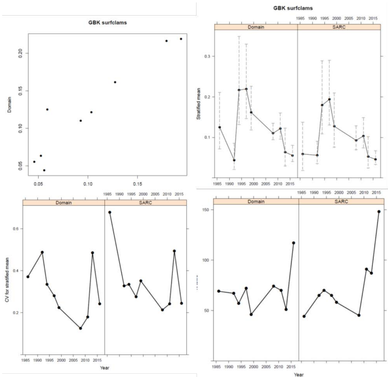
Figure 36. Post-stratified means, 95% confidence intervals, and coefficient of variation (CV) based on domain variance calculations and sample size (N tows) for Georges Bank (GBK) Atlantic surfclams ( Spisula solidissima ) calculated using recommended (Domain) and current Stock Assessment Review Committee (SARC) stratification schemes.
