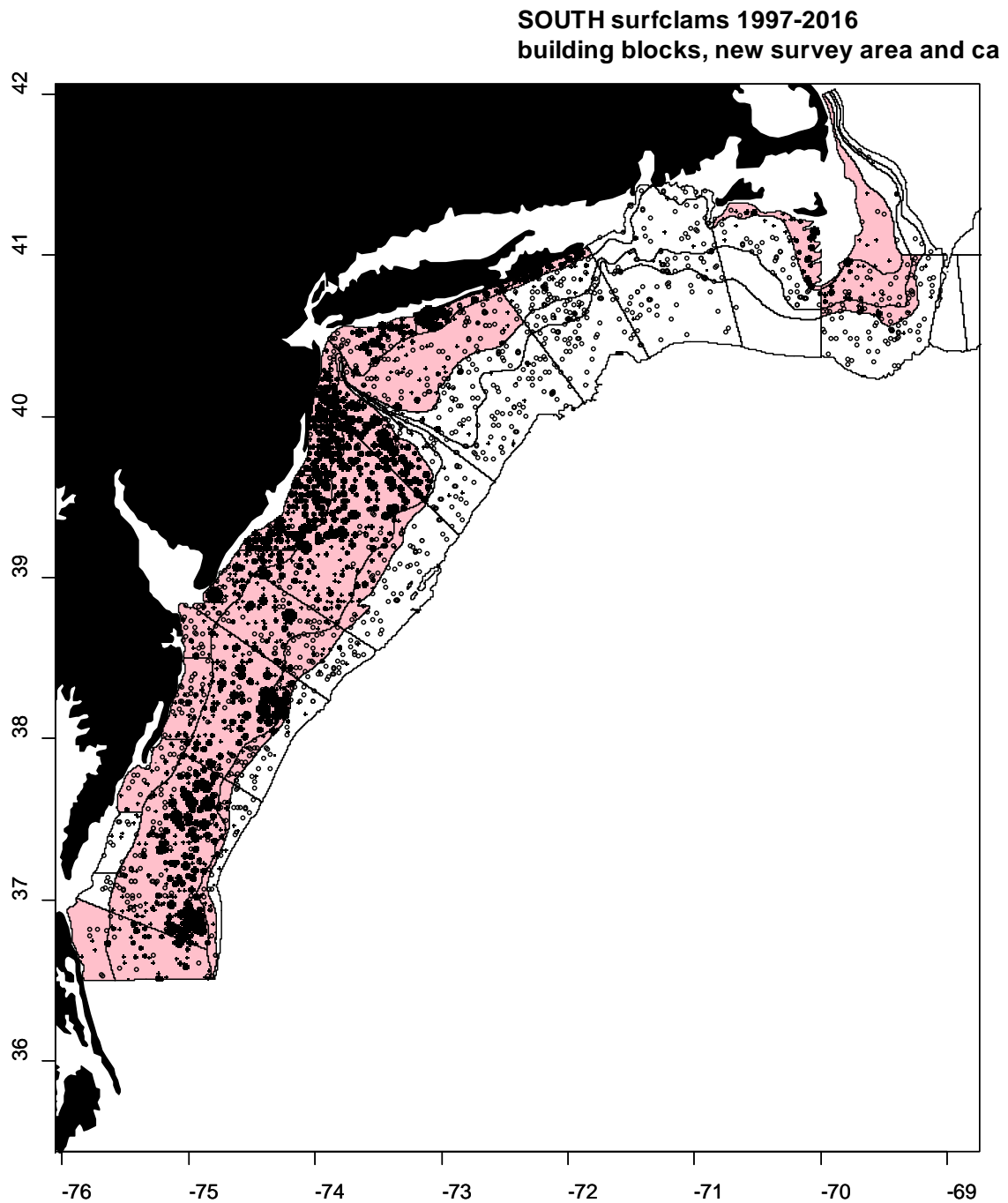
Figure 12. New building blocks (lines) and survey area (shaded) based on the 1% rule for surfclams ( Spisula solidissima ) in the southern areas, with survey data from 1997-2016 (rescaled to same annual mean). Hollow symbols show stations with zero catch. Solid symbols show location amount and location of catches.
