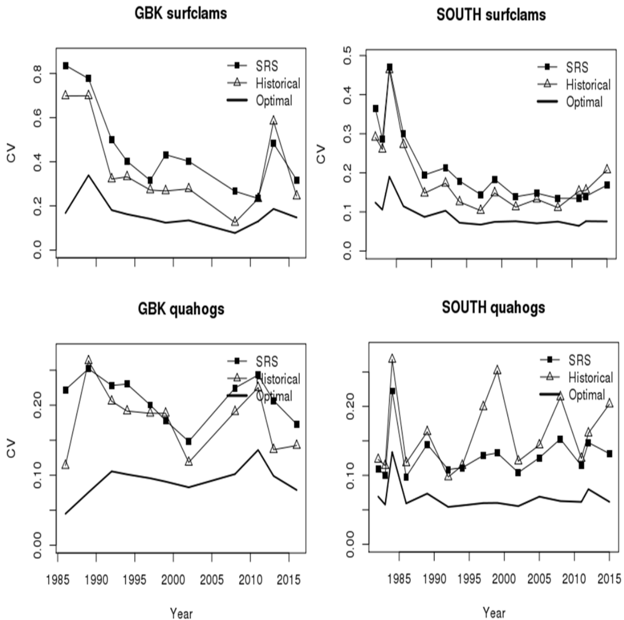
Figure 15. Historical analysis showing coefficient of variation (CV) for stratified mean catch density in Northeast Fisheries Science Center (NEFSC) clam surveys based on the current design and CVs expected under random sampling and with optimal allocation for Atlantic surfclam ( Spisula solidissima ) and ocean quahog ( Arctica islandica ) in Georges Bank (GBK) and the southern assessment areas. All 3 scenarios use the current stratification scheme.
